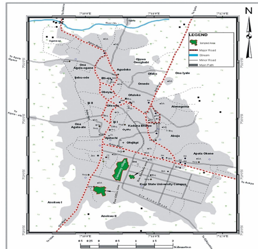
Figure 1: Map of Anyigba showing the sampled areas (Source)
