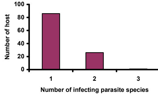
Figure 7: Multiple parasitic infections of Amietophrynus regularis
