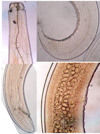
Figure 3: Amplicaeum africanum infecting Amietophrynus regularis . (A) anterior end, (B) male posterior end, (C) female posterior end, (D) vulva region of female with ovary showing eggs
