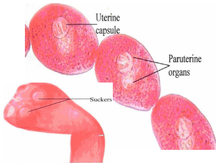
Figure 2: Baerietta jaegerskioeldi infecting Amietophrynus regularis
